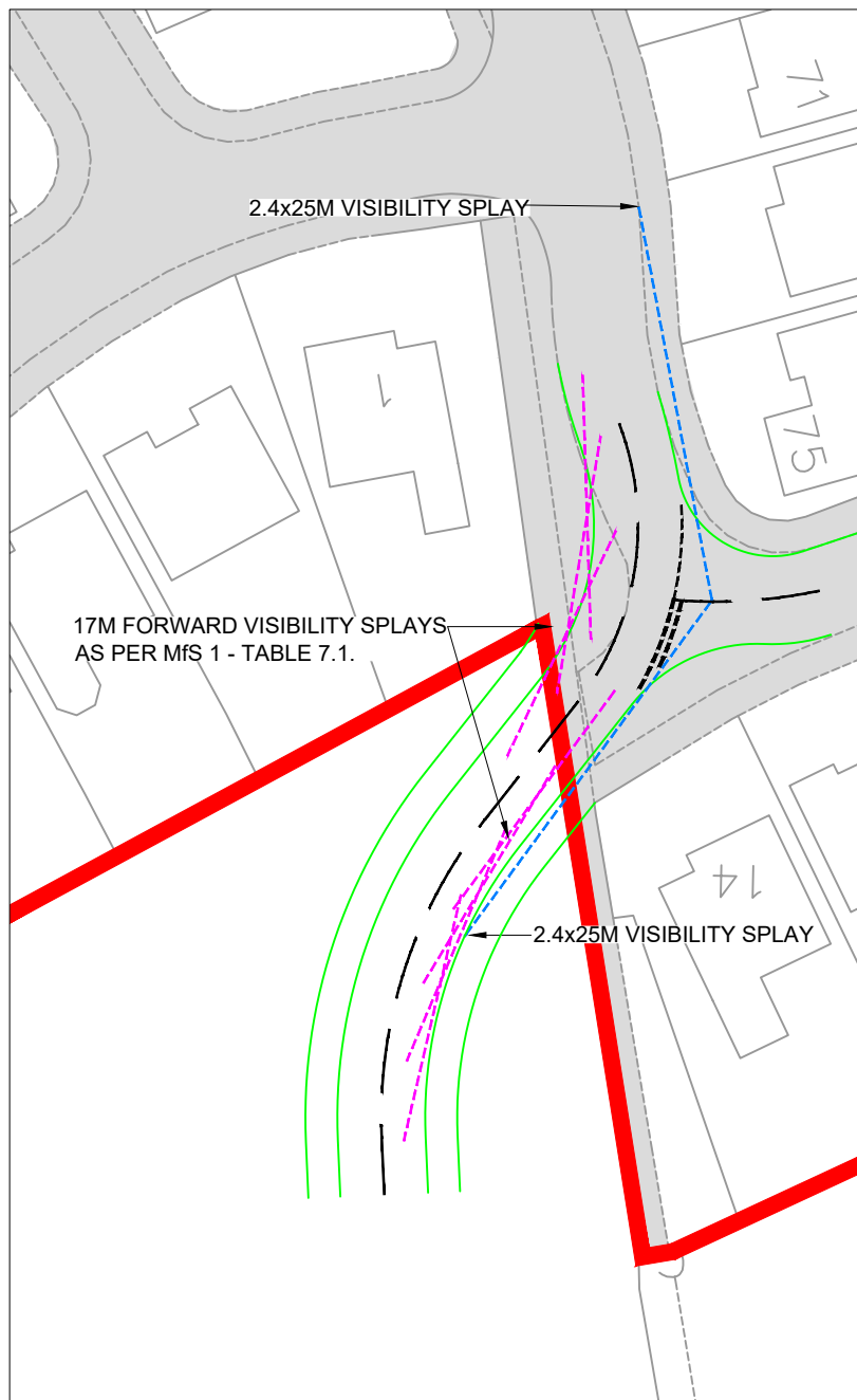
VISIBILITY SPLAYS
